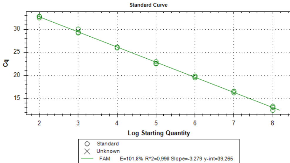
Figure 3: Standard curve for Yellow stripe virus
