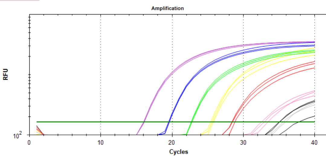
Figure 1: Logarithmic amplification curves for Salmon Pancreas Disease Virus
