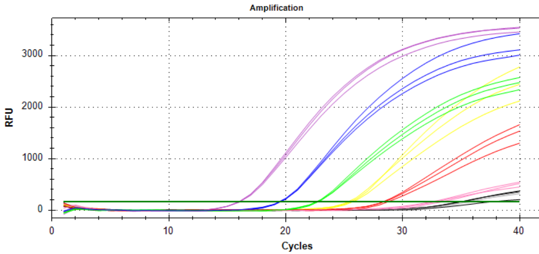
Figure 2: Standard amplification curves for Salmon Pancreas Disease Virus
