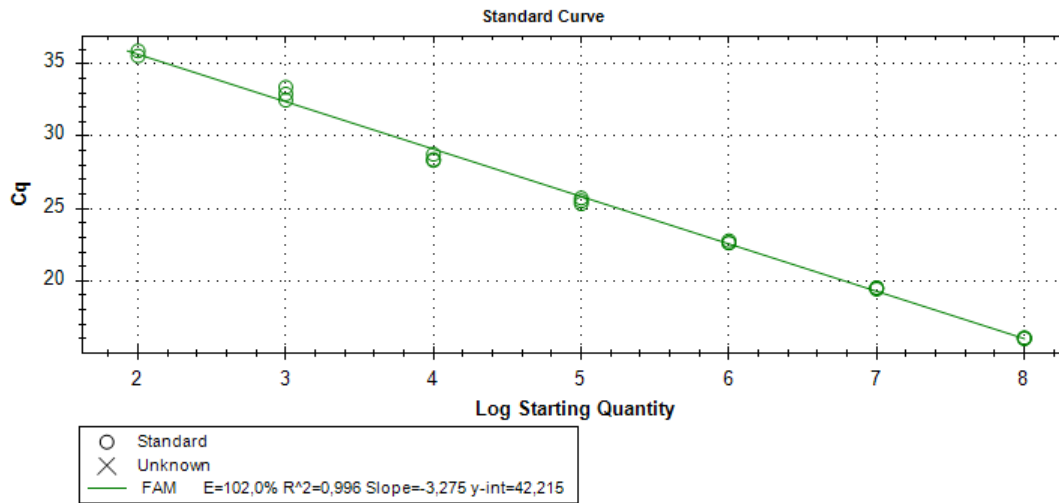
Figure 3: Standard curve for Salmon Pancreas Disease Virus
