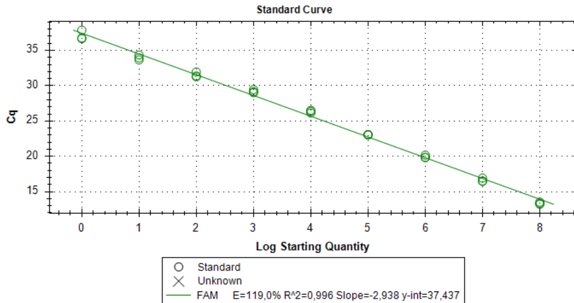
Figure 3: Standard curve for Olive Latent Virus-1
