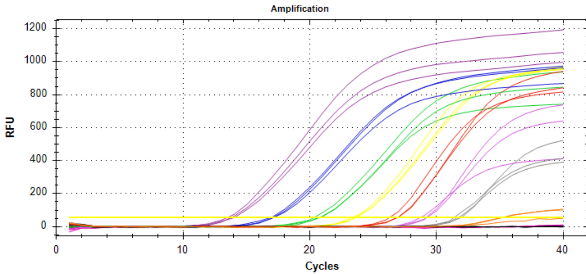
Figure 2: Standard amplification curves for Yersinia pseudotuberculosis
