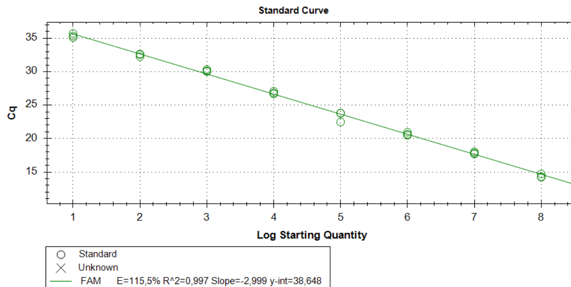
Figure 3: Standard curve for Meloidogyne spp.
