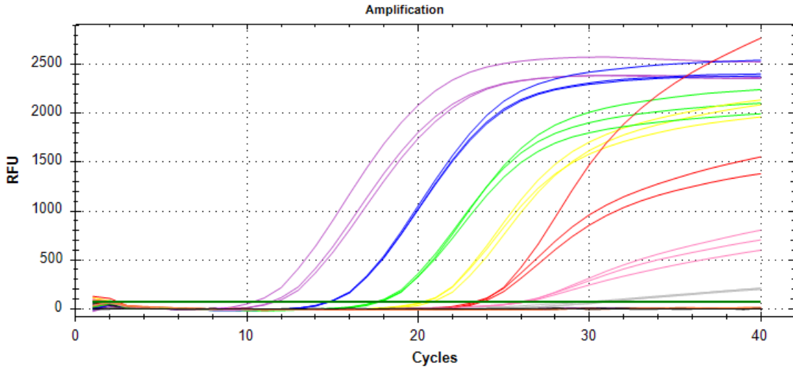
Figure 2: Standard amplification curves for Helicobacter spp.
