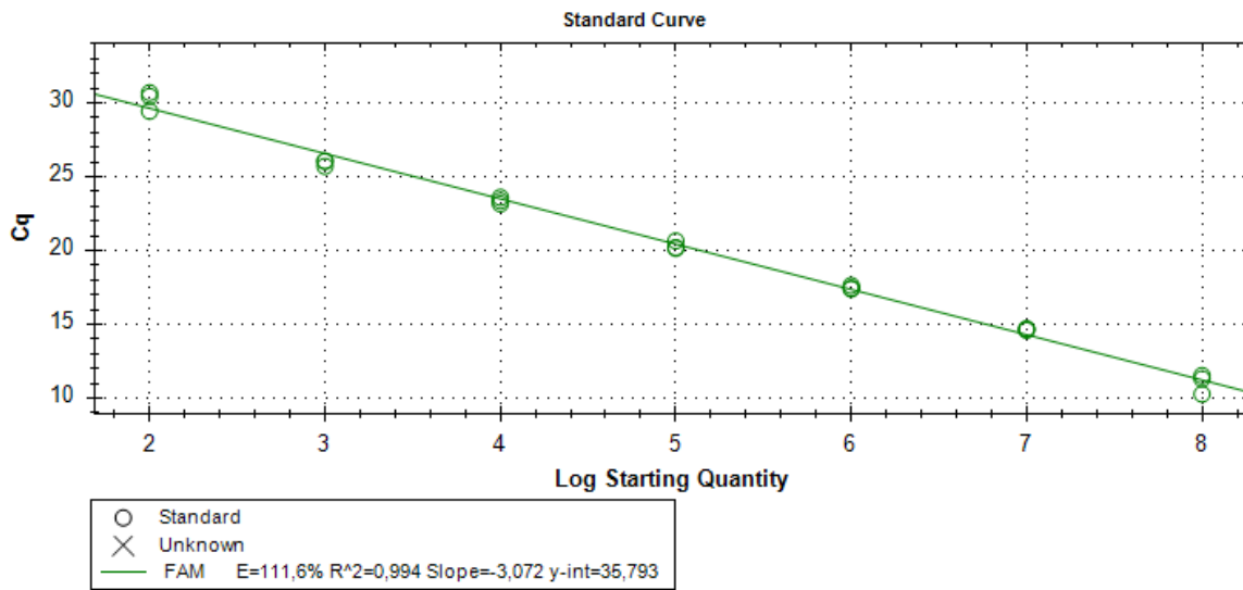
Figure 3: Standard curve for Helicobacter spp.
