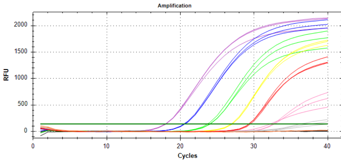
Figure 2: Standard amplification curves for Globodera rostochiensis
