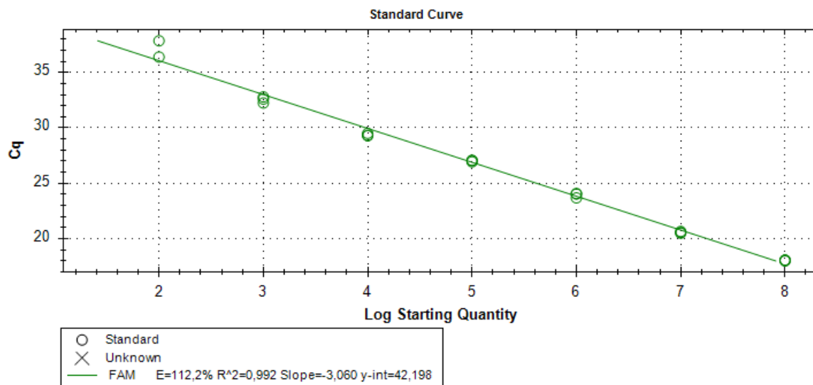
Figure 3: Standard curve for Globodera rostochiensis
