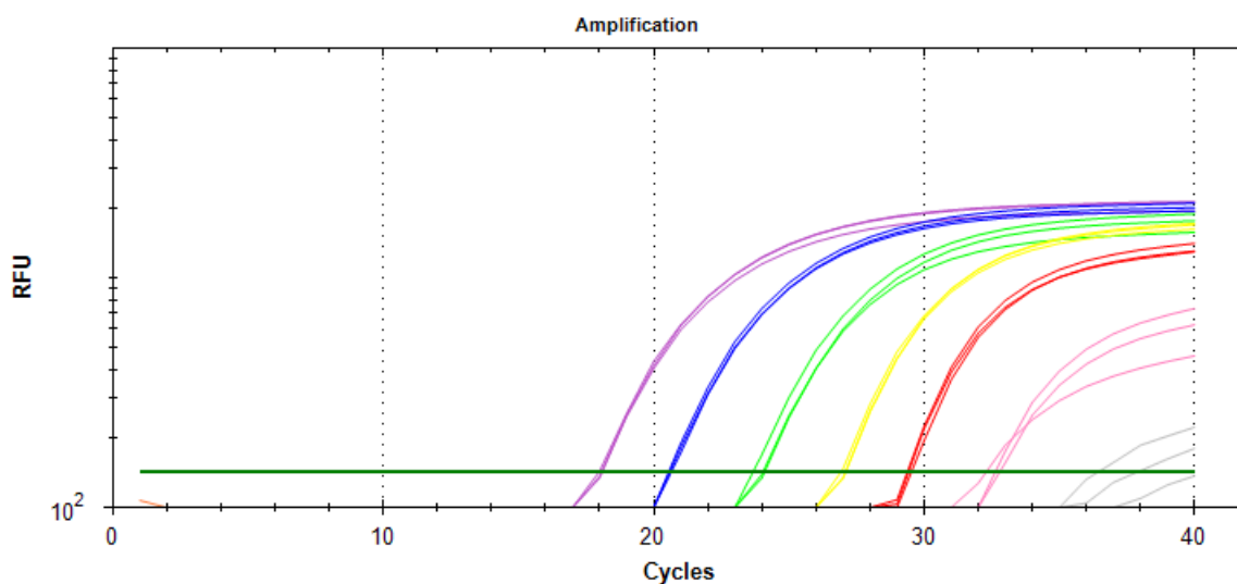
Figure 1: Logarithmic amplification curves for Globodera rostochiensis
