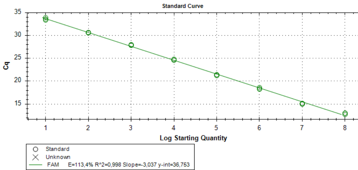
Figure 3: Standard curve for Fusarium oxysporum f. sp. cubense
