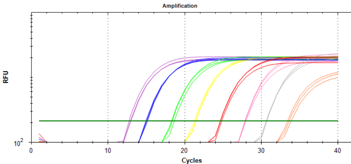
Figure 1: Logarithmic amplification curves for Fusarium oxysporum f. sp. cubense
