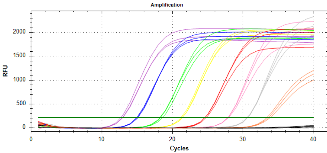
Figure 2: Standard amplification curves for Fusarium oxysporum f. sp. cubense
