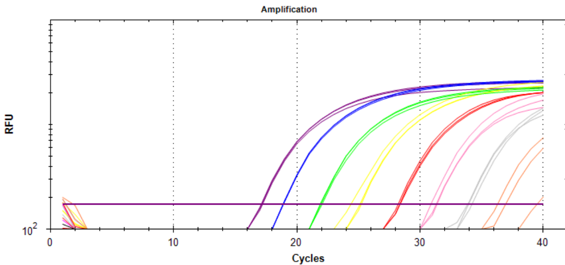
Figure 1: Logarithmic amplification curves for Ebola Bundibugyo virus
