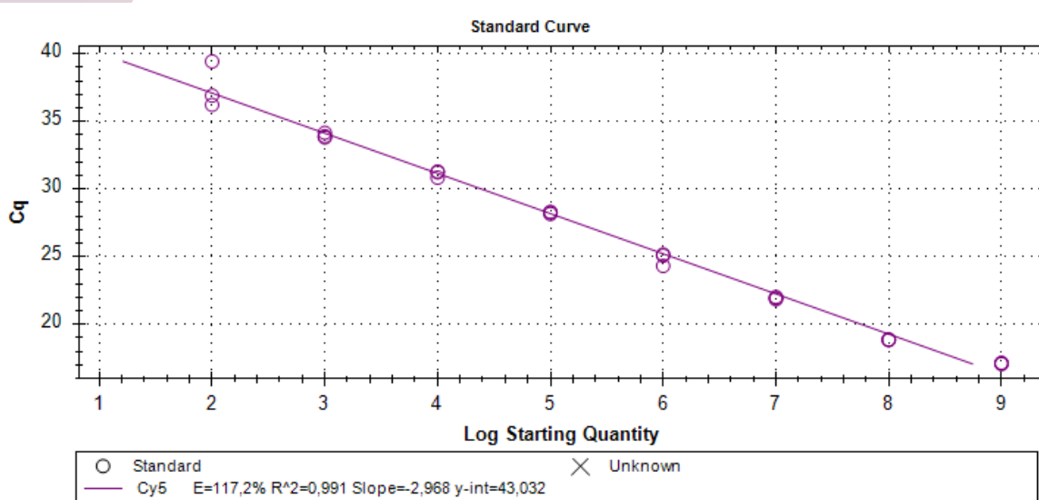
Figure 3: Standard curve for Ebola Bundibugyo virus
