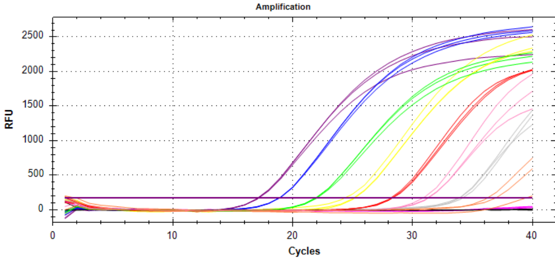
Figure 2: Standard amplification curves for Ebola Bundibugyo virus
