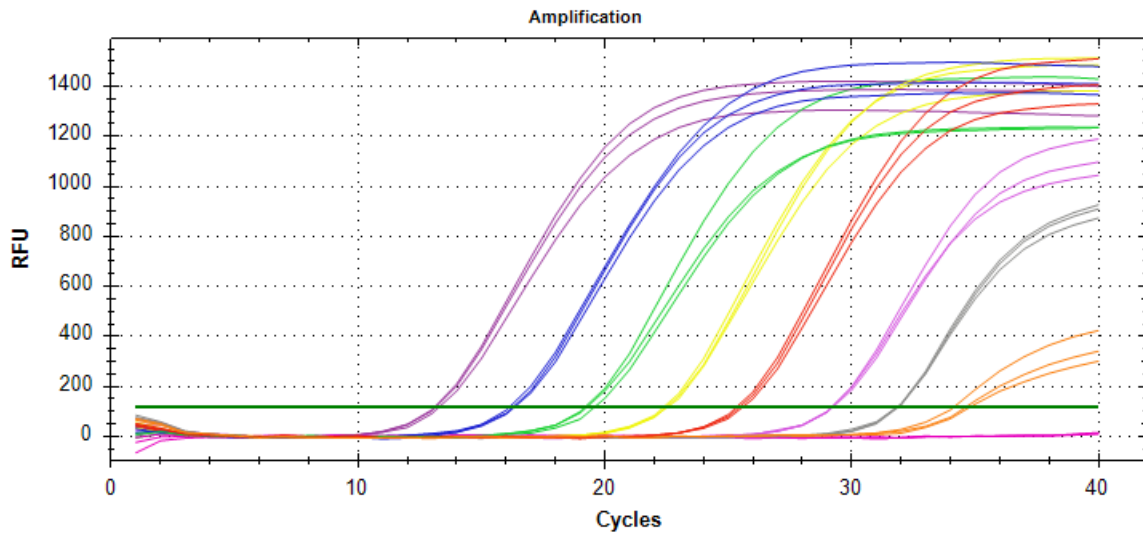
Figure 2: Standard amplification curves for Clostridium estertheticum
