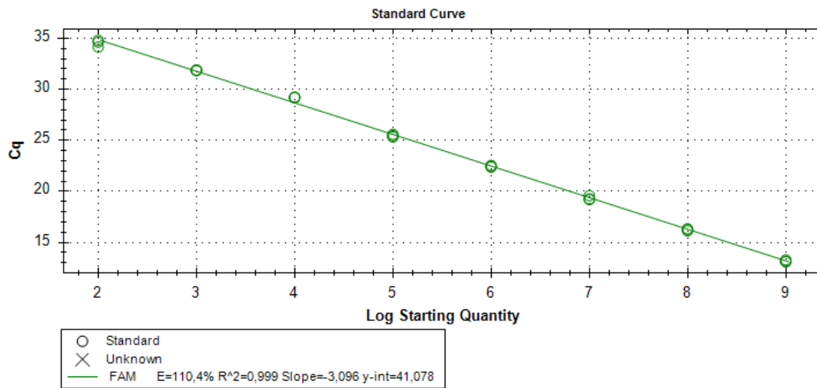
Figure 3: Standard curve for Clostridium estertheticum
