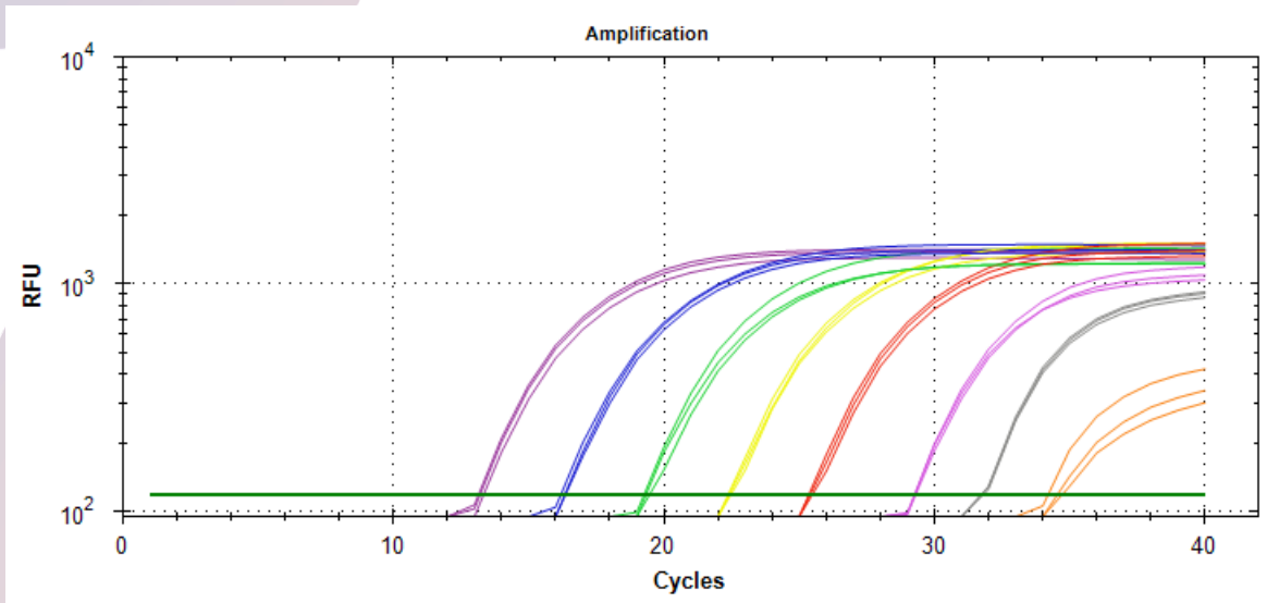
Figure 1: Logarithmic amplification curves for Clostridium estertheticum
