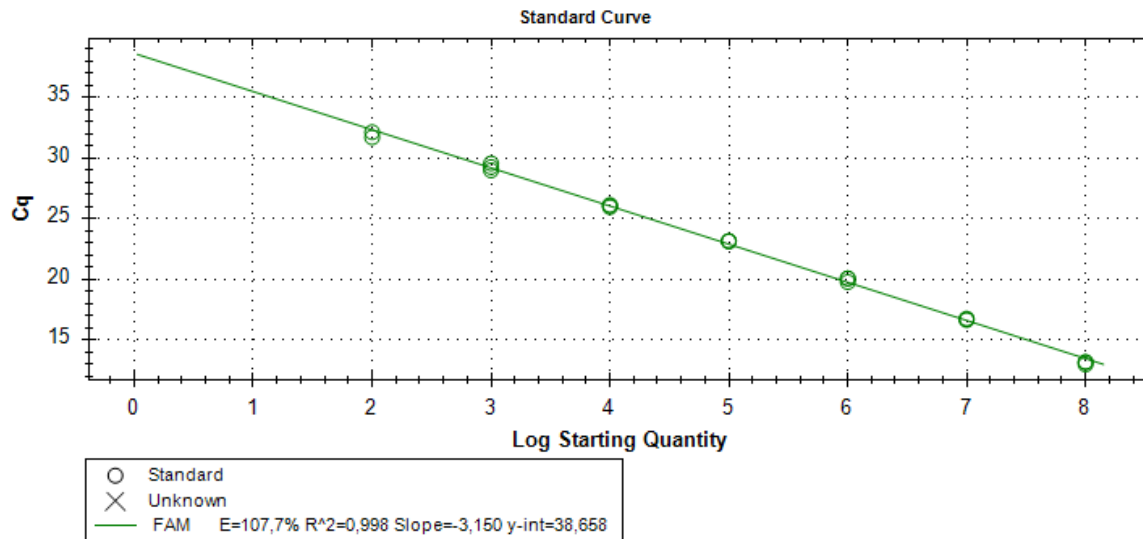
Figure 3: Standard curve for Chlamydomonas psittaci abortus
