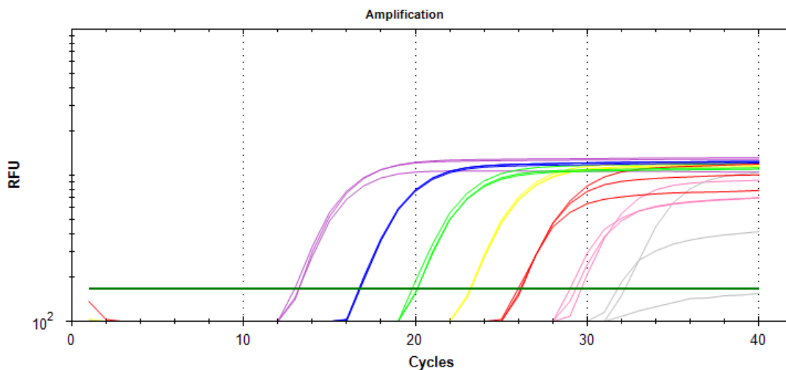
Figure 1: Logarithmic amplification curves for Chlamydophila psittaci abortus
