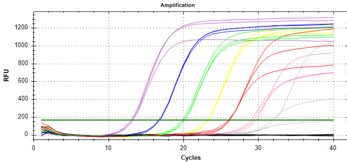
Figure 2: Standard amplification curves for Chlamydomonas psittaci abortus
