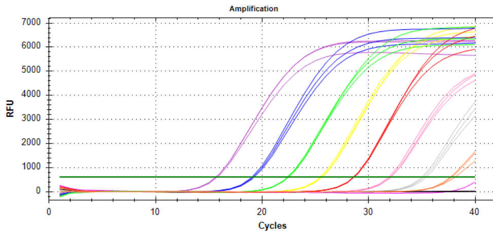
Figure 2: Standard amplification curves for Lumpy skin virus
