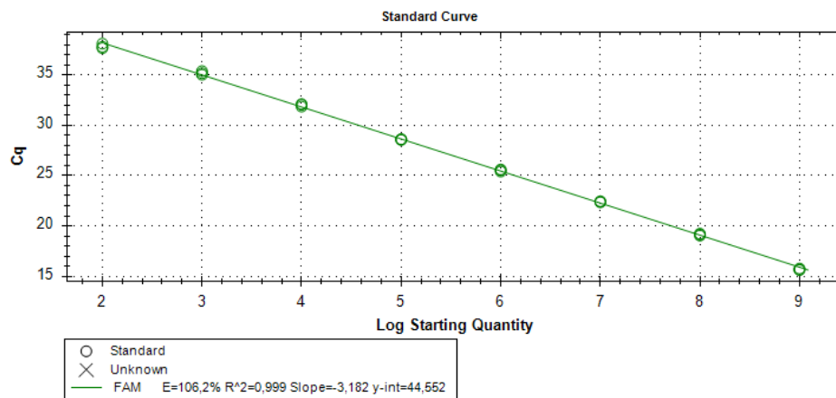
Figure 3: Standard curve for Lumpy skin virus
