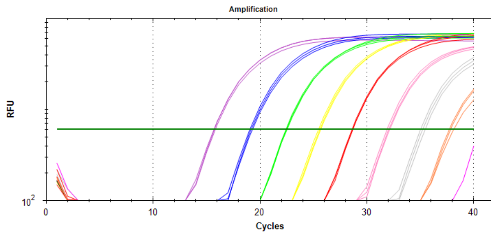
Figure 1: Logarithmic amplification curves for Lumpy skin virus
