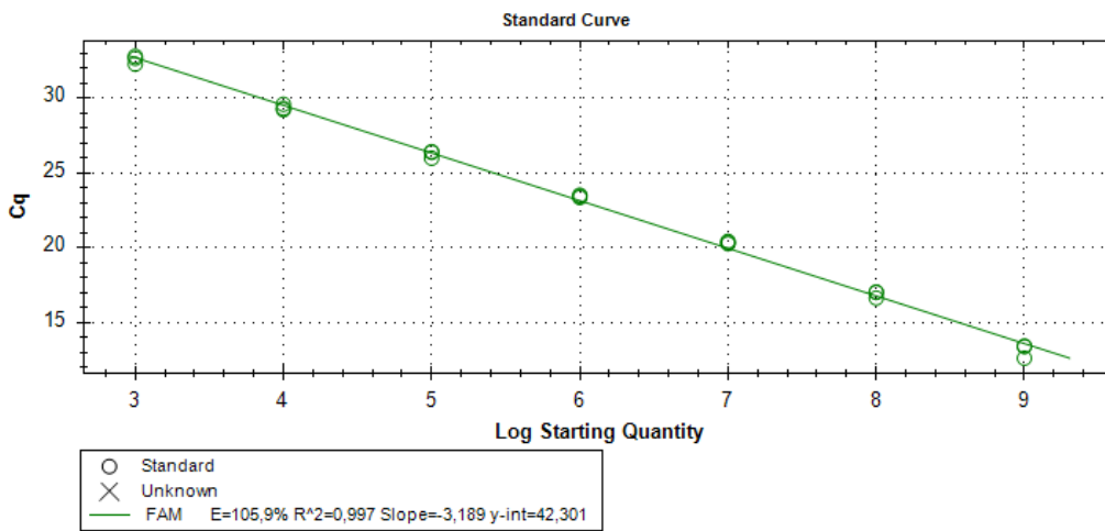
Figure 3: Standard curve for Botryphaeriaceae
