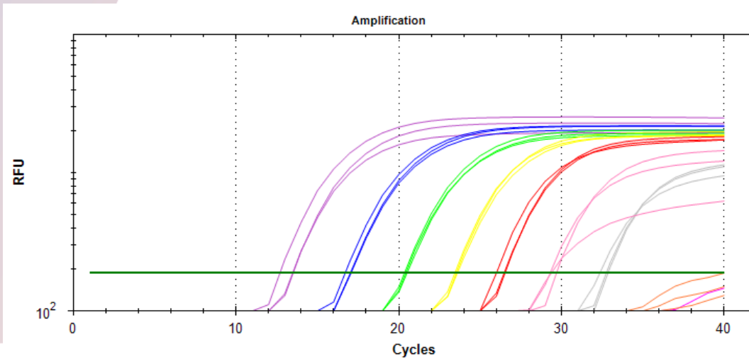
Figure 1: Logarithmic amplification curves for Botryophaeeriaceae
