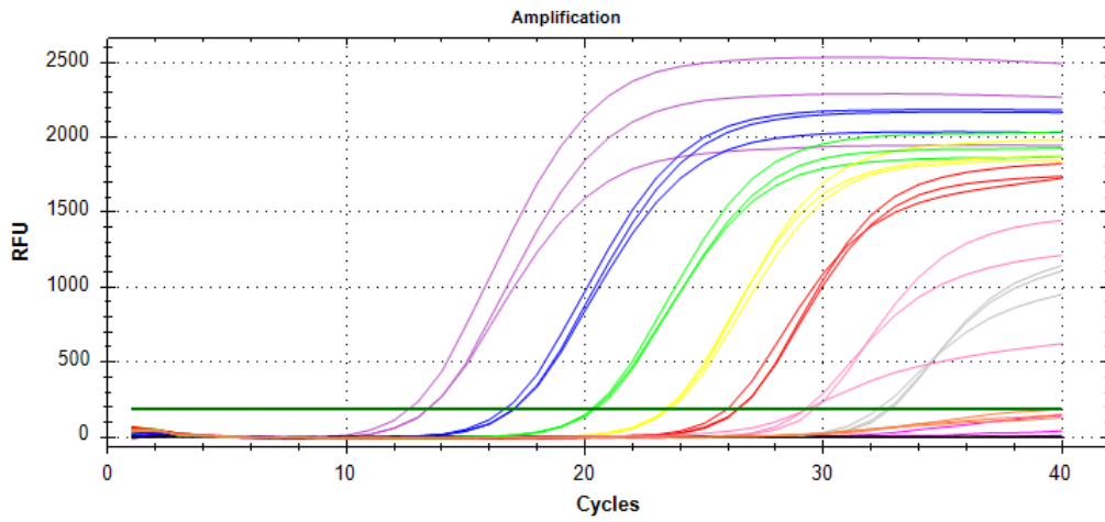
Figure 2: Standard amplification curves for Botryphaeriaceae
